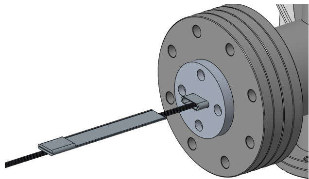
Figure 3: Concept of the Hall sensor carriage that slides within the guide tube.
