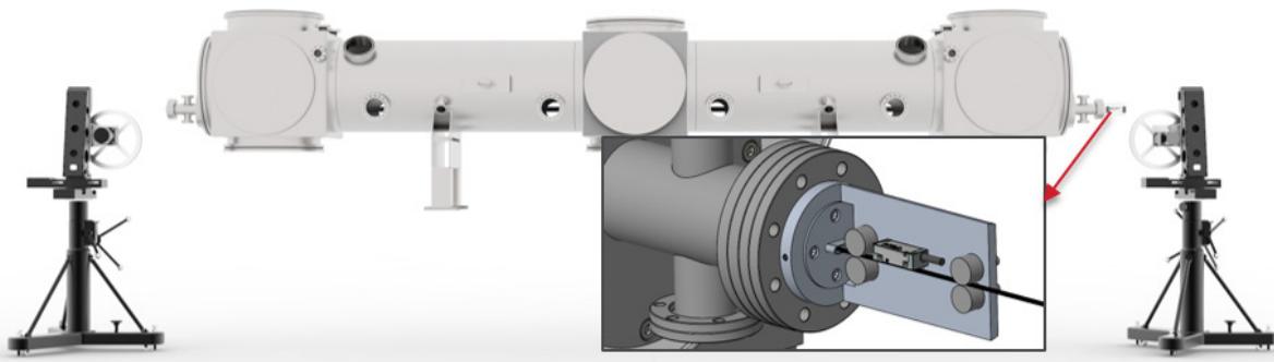
Figure 2: Measurement system installed at the ends of the SCU production cryostat. The inset is a close view of the encoder linear scale and stationary read head assembly.
