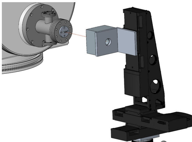
Figure 4: Rotary stage installed on the 3-axis stage assembly for wire-based measurements.
