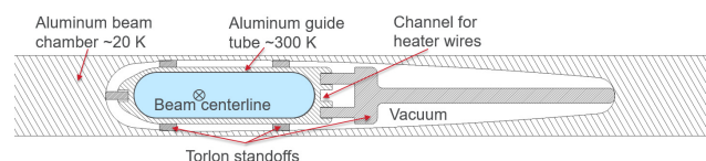
Figure 1: Cross section of the guide tube placement inside the beam vacuum chamber.
